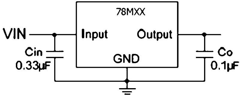
Fig.1 Fixed Output Regulator
